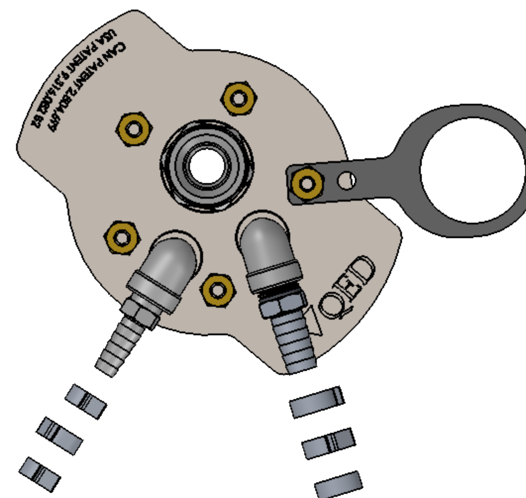
AS ASSEMBLED
