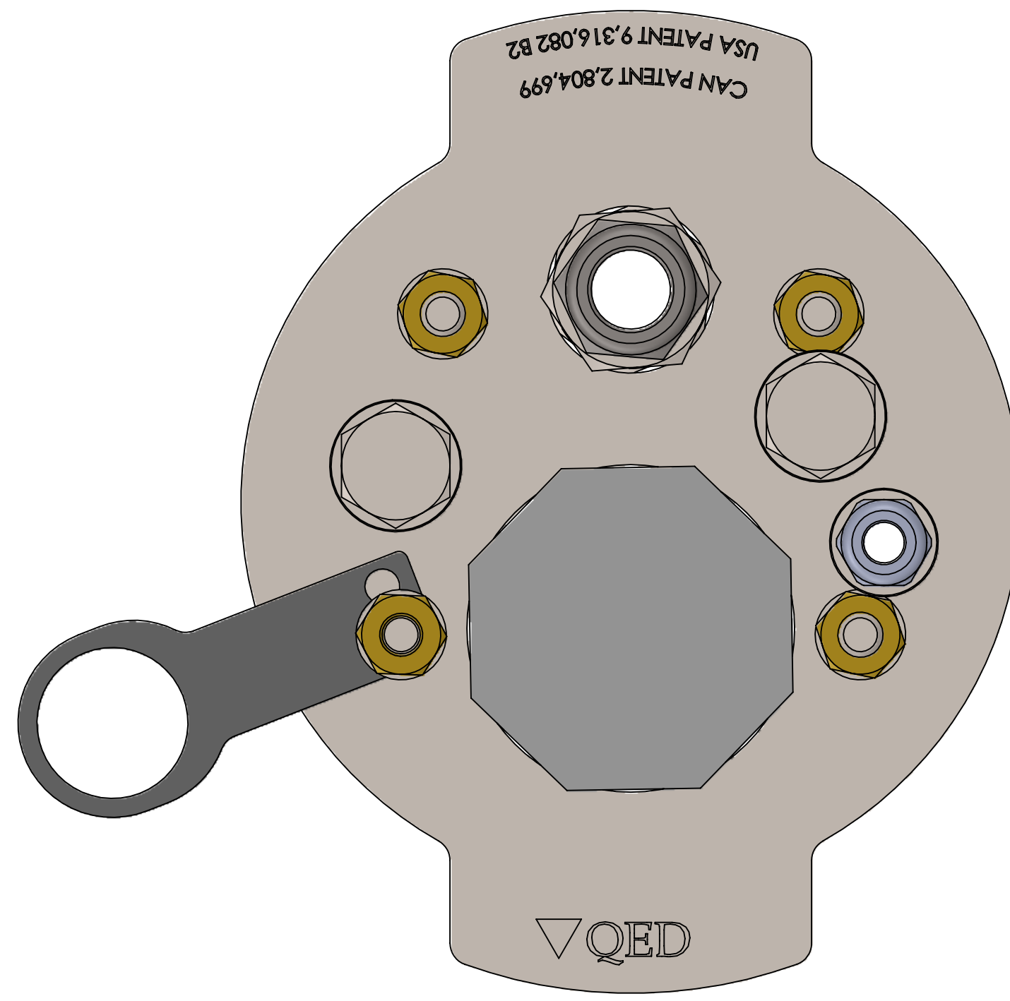
AS ASSEMBLED
